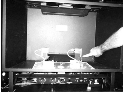
Figure 2: Accent light bracket screws location
