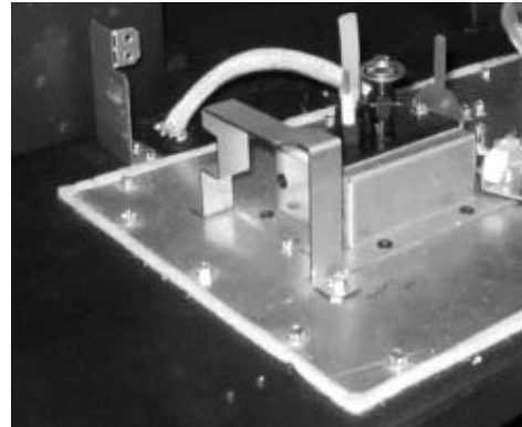
Figure 6: Burner support bracket installed
