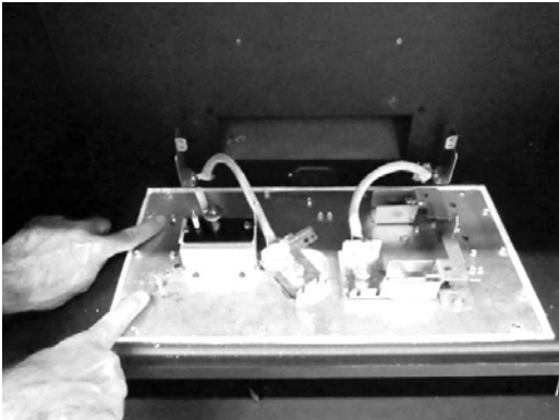
Figure 5: Burner support bracket screws location
