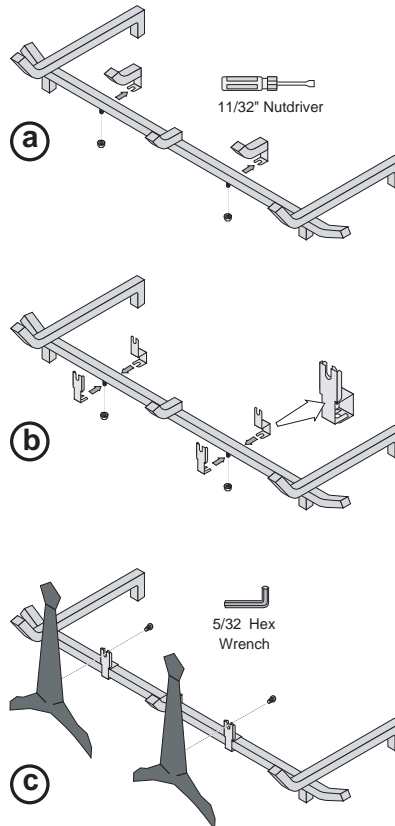
Figure 1: Andiron Clips Installation
