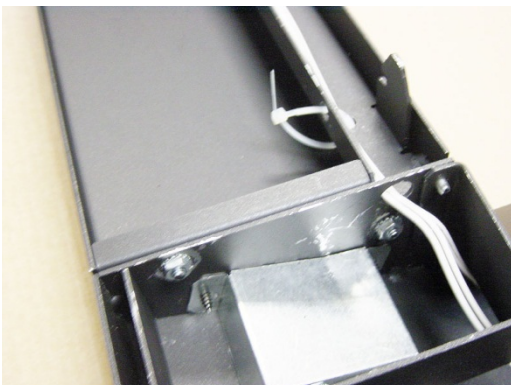
Figure 7: Wires secured with lock-tie
