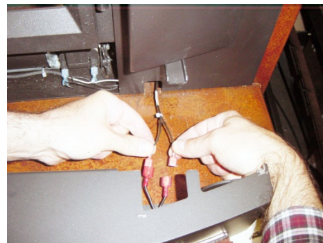
Figure 16: Connecting the bottom right wires
