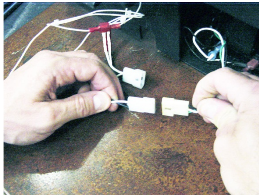
Figure 10: Connecting the Molex connectors
