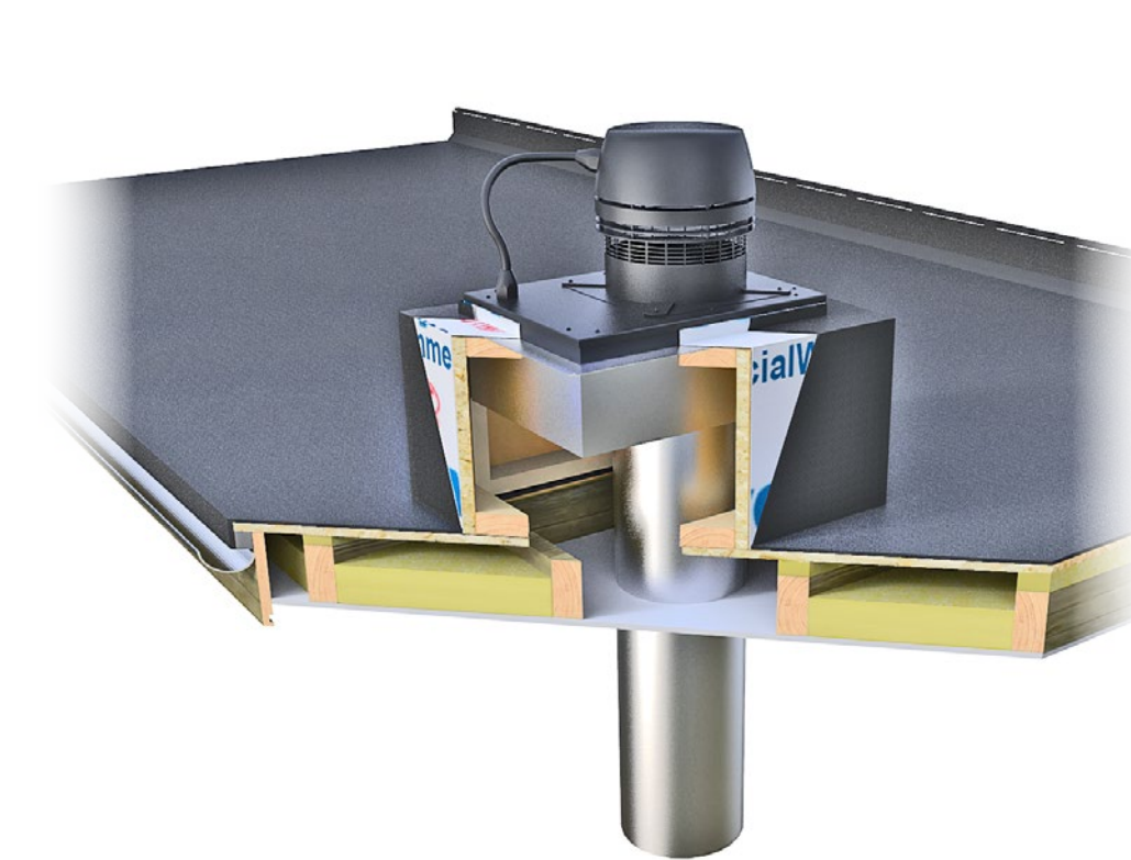
Vertical (Roof Top) Power Exhaust Vent Fan Termination
