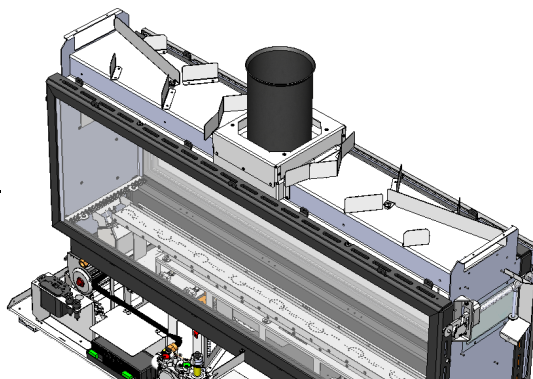
Cutaway of Air Diverter
